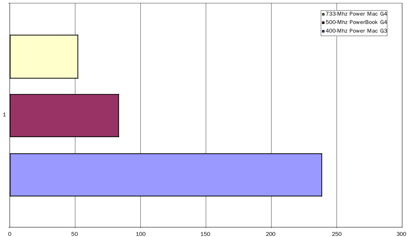
Adobe Photoshop Performance - 70 MB File - Total Time (Time in seconds - shorter is better)
