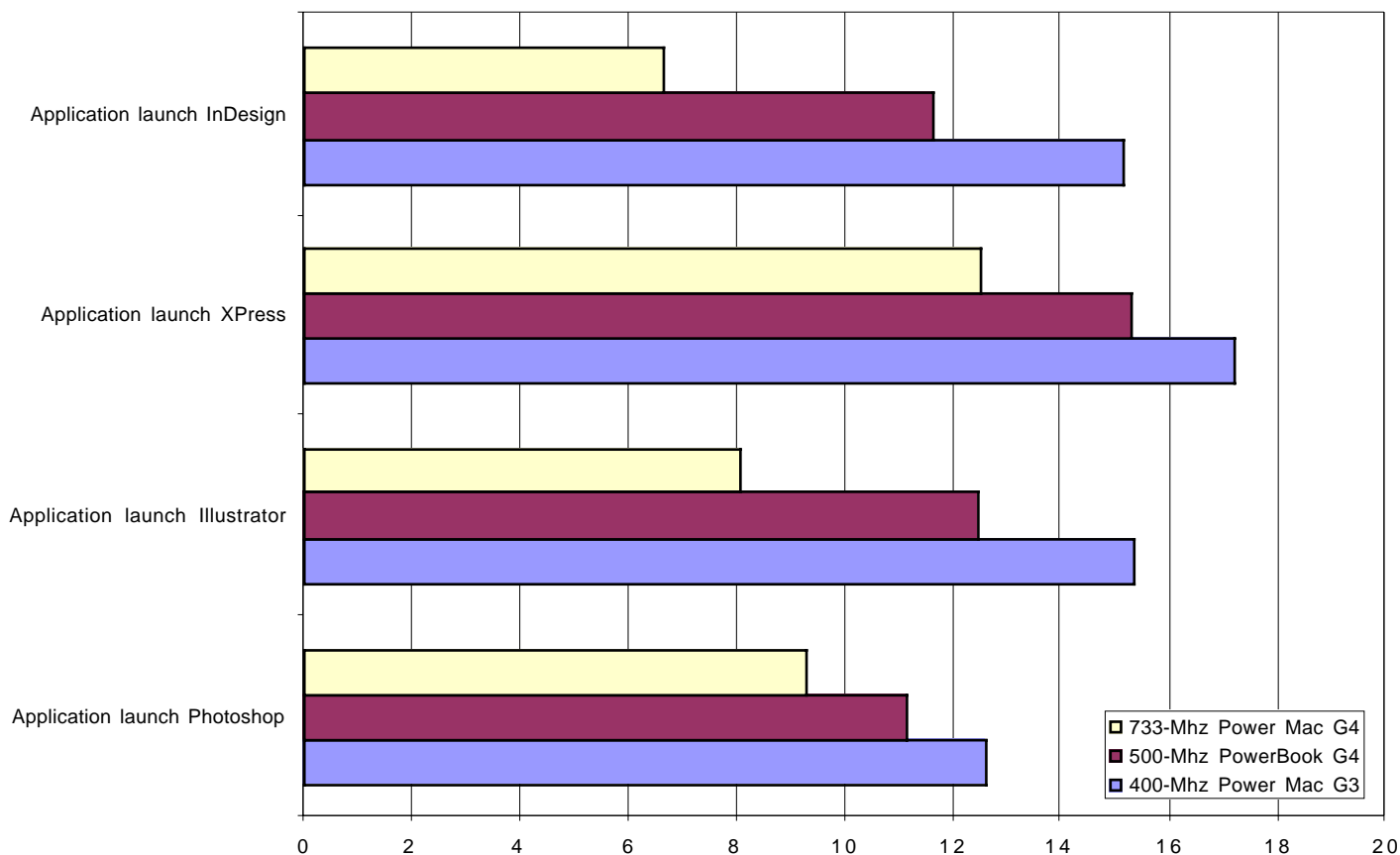
System Performance 2 - Application Launch (Time in seconds - shorter is better)
