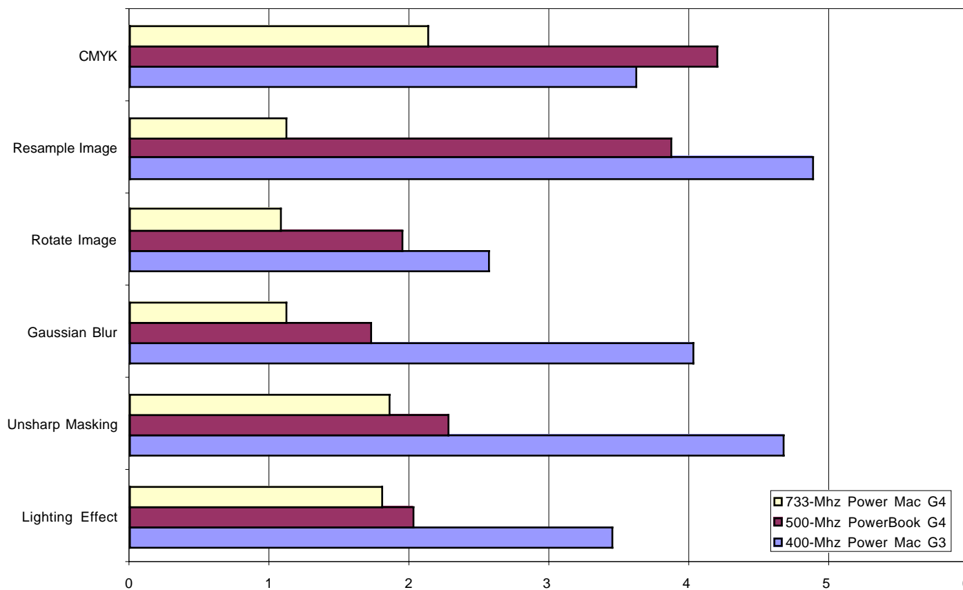
Adobe Photoshop Performance - 5 MB File (Time in seconds - shorter is better)
