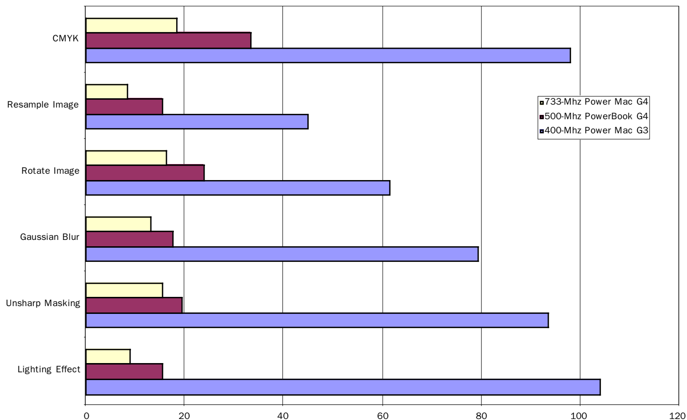
Adobe Photoshop Performance - 70 MB File (Time in seconds - shorter is better)
