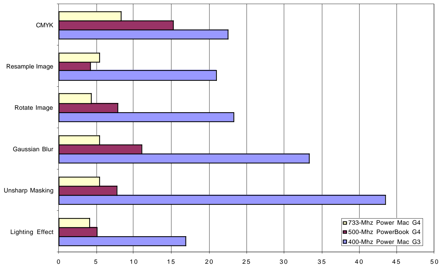
Adobe Photoshop Performance - 30 MB File (Time in seconds - shorter is better)
